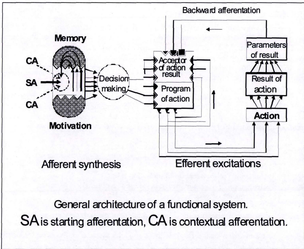
Figure 2: Architecture of Functional System in Central Nervous System by P. K. Anokhin (redrawn from the article of Red'ko V.G. et al., [20] with the permission of the authors).
