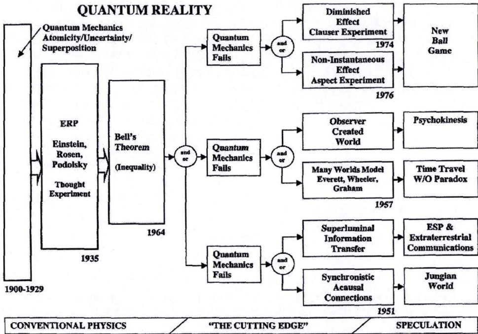
Figure 4. Historical development of the quantum theory.
