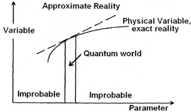
Figure 2. We approximate the quantum domain as a linear variable dependent on a parameter. The full "space" of exact reality is nonlinear.
