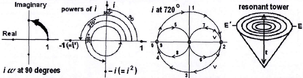
Figure 9. Powers of i in the complex plane. For 90° to 360° the concept can be readily illustrated in 2D; but for 720° and above 4D is required which cannot easily be depicted in 3D so the representation in 9c) is used, which might also be represented by a Klein bottle which was not used because the torus in 9c) more easily shows the rotation topology, which for spin 1/2 is the Dirac rotation of the electron. 9d) is a simplistic representation of a powers of i resonance hierarchy.
