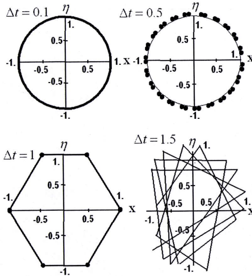
Figure 5. Numerical simulation of the phase space trajectory of the Dubois superposed incurvise oscillator based on coordinates and velocities x_n = 1/2[x_n(1) + x_n(2)] v_n = 1/2[v_n(1) + v_n(2)] is shown in the figure for values of \Delta t = \omega t equal to 0.1, 0.5, 1.0 and 1.5. Initial conditions are x_0 = 1, \eta_0 = 0 & t_0 = 0 with total simulation time t = \omega t = 8\pi . Figure adapted from [45].
