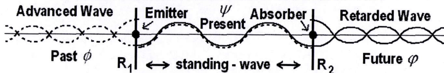
Figure 11. Structure of a transaction (present state or event) where the present is a standing-wave of future-past elements. The separation of these parameters in terms of de Broglie's fusion model is suggested to allow manipulation of the harmonic tier of the L.O.V.E.R.
