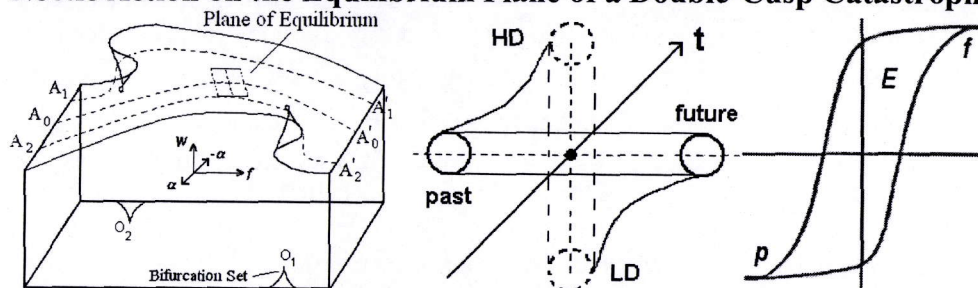
Figure 3. a) The DCC is illustrated showing cusps at each end of the plane of equilibrium. The DCC is said to occur in \geq 9 dimensions and thought to be the catastrophe form most compatible with the symmetry of NFT. The spacetime component of the plane of equilibrium is a topological manifold tiled of noetic least units . The equilibrium manifold undergoes a 'conscious' quantum computation best described by interactive computation. b) Graphically illustrates the fundamental scale invariant noetic equation F_N = E/R of conscious action, the basis of the noetic effect on the plane of equilibrium. c) The hysteresis loop of the Hamiltonian mapped out by the future-past parameters of noetic spacetime. The area E represents the energy of the noetic force F_N .
