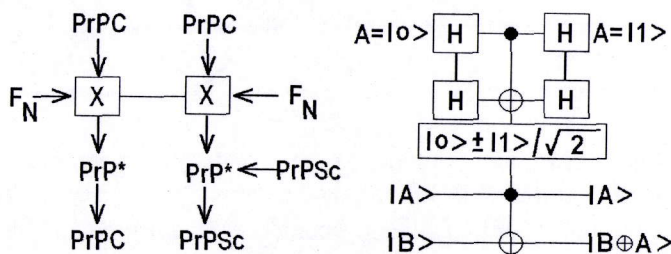
Figure 1. a) Flow chart for Prion propagation, where factor-X is postulated to be the action of Noetic Field, F_N . b) Circuit representation for a possible quantum logic gate configuration for \text{PrP}^C Propagation. Two Hadamard gates, H generate a superposed intermediate conformation of \text{PrP}^C called \text{PrP}^* in state |0\rangle \pm |1\rangle / \sqrt{2} , illustrating the possibility that the Prion's pathological process acts a quantum Hadamard Controlled-Not Gate; |A\rangle is the control qbit and |B\rangle is the target qbit.
