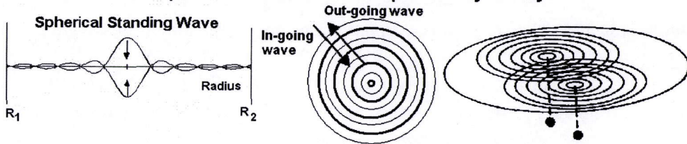
Figure 4. The Dirac polarized vacuum has hyperspherical symmetry. a) Metaphor for standing-wave present showing future-past elements, R_1, R_2 , eleven of twelve dimensions suppressed for simplicity. b) Top view of a) a 2D spherical standing-wave. c) Manipulating the relative phase of oscillations creates nodes of destructive and constructive interference.
