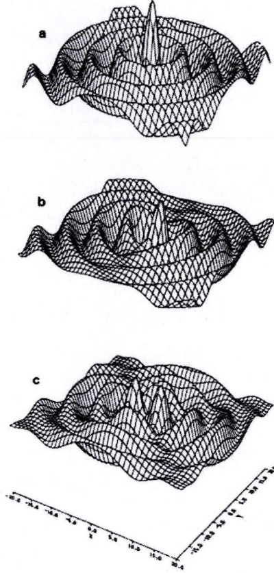
Figure 1: Variation of the real component of the transverse wave, \psi_T = J_n(\ell r) e^{i n \theta} , is plotted as a function of the coordinates on the transverse plane (represented here as the horizontal X,Y plane). Here, X = \ell r \cos \theta and Y = \ell r \sin \theta . (a) n = 0 , (b) n = 1 , and (c) n = 2 .
