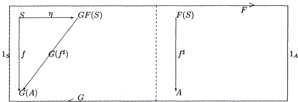
Fig. 7: Distinction of f^\# in S by arrow G(f^\#)
