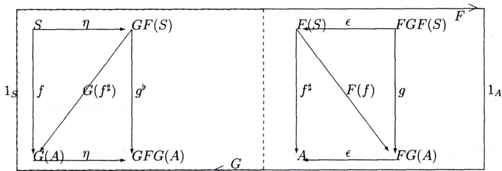
Fig. 12: Correlation between Arrow g in A and g^b in S where \eta > 0 and \epsilon < 1
