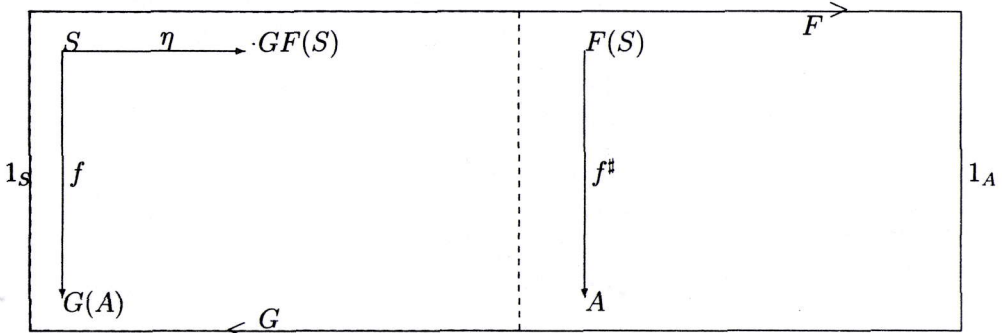
Fig. 6: Correlation between Arrow f in S and f^\# in A where \eta > 0
