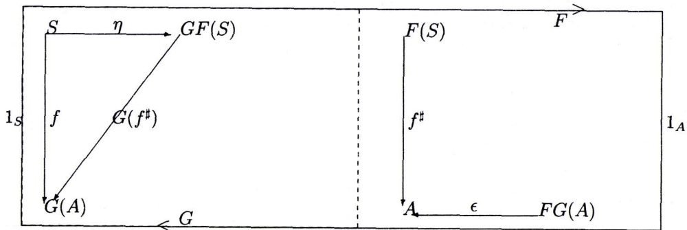
Fig. 9: Correlation between Arrow f in S and f^\# in A where \epsilon < 1
