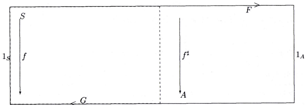
Fig. 4: Correlation between Arrow f in S and f^\# in A
