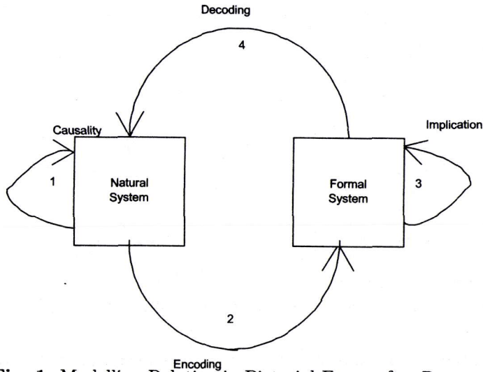
Fig. 1: Modelling Relation in Pictorial Form, after Rosen
