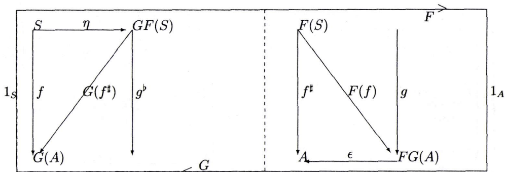
Fig. 11: Correlation between Arrow g in A and g^b in S
