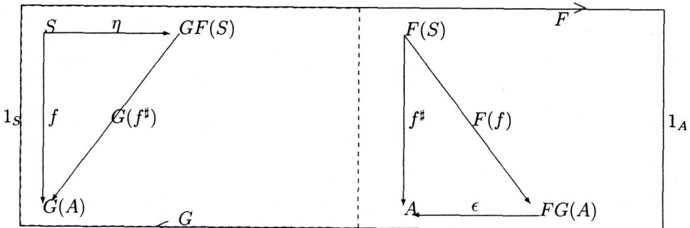
Fig. 10: Distinction of f in A by arrow F(f)
