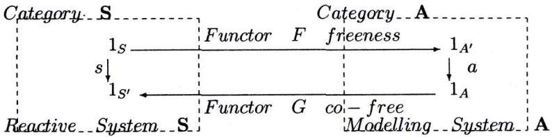
Fig. 14: Nature of Modelling Systems: \eta = 0 and \epsilon = 1
