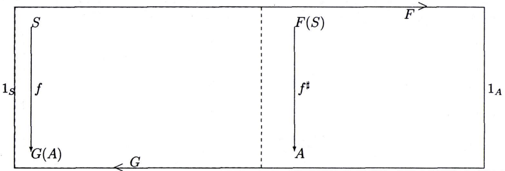
Fig. 5: Correlation between Arrow f in S and f^\# in A where \eta = 0
